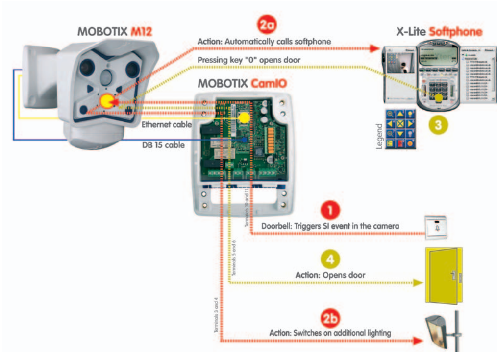
Sample: Door intercom system with Video SIP and additional lighting
